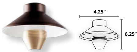
6" Brass Path/Area Hat (D6PTH-HAT)
